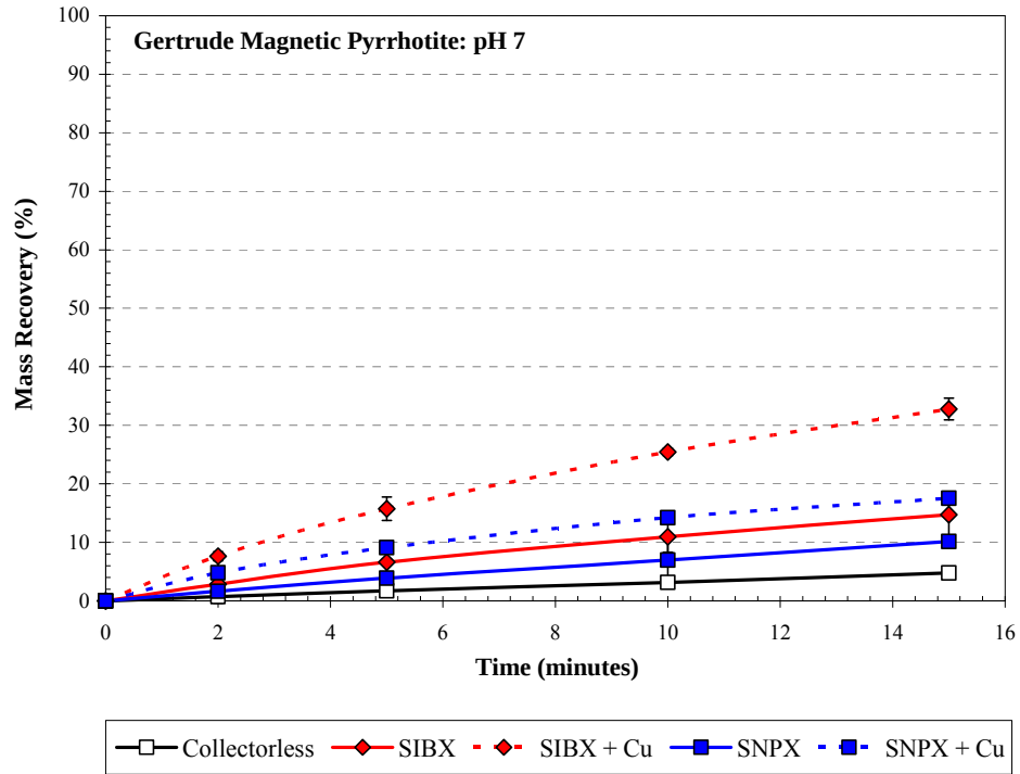
Figure 6.11: Mass recovery versus time from microflotation tests of Sudbury Gertrude magnetic pyrrhotite at pH 7. The 2\sigma standard deviation is also shown.
