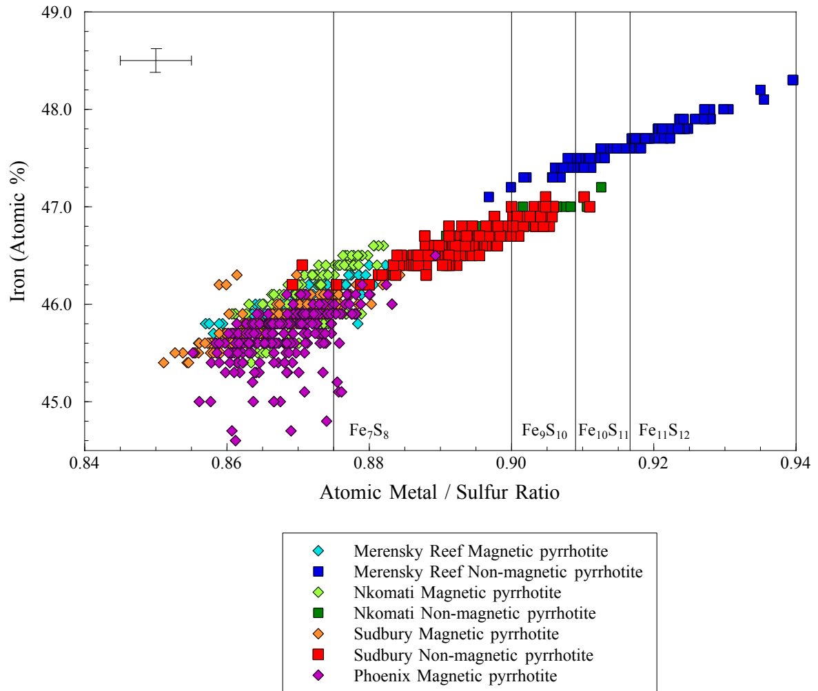
Figure 4.22: Comparison of the atomic % iron versus metal to sulfur ratio for all magnetic and non-magnetic pyrrhotite occurrences examined in this study. The 2σ standard deviation is also shown.
