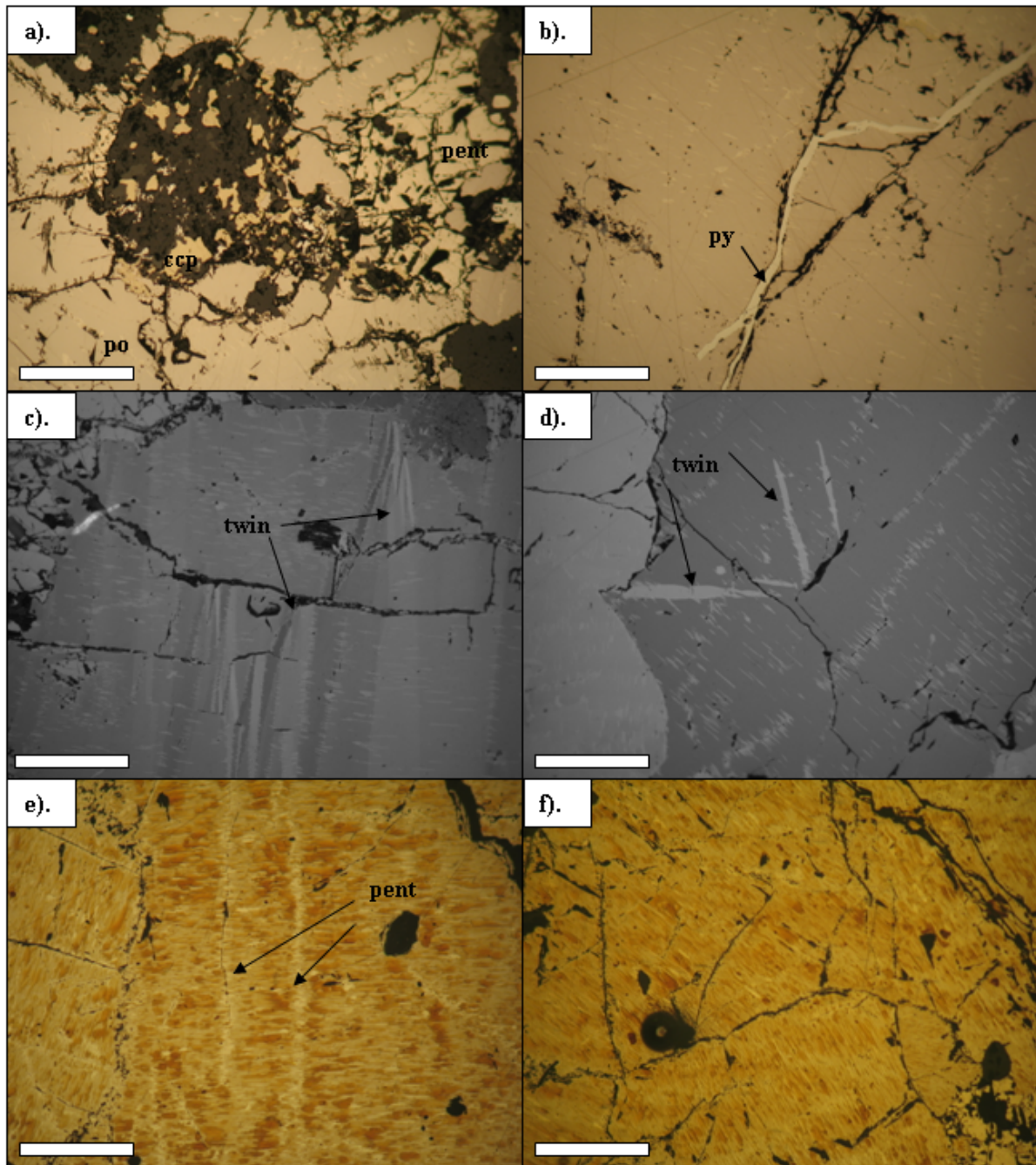
Figure 4.5: Photomicrographs of the Phoenix massive sulfide ore shown in RPL and XPRL (c, d). (a) Silicate inclusion hosted by the massive sulfide. Note the resorbed nature of the pyrrhotite hosting the silicate inclusion. (b) Pyrite vein hosted by pyrrhotite, which in turn hosts multiple flame pentlandite lamellae. (c, d) Twinning in pyrrhotite. Feathered textures belong to the flame pentlandite lamellae. (e, f) Magnetic colloid treatment shows Phoenix pyrrhotite is magnetic. Note the exsolution of flame pentlandite parallel from a fracture, coincident to the direction of magnetic pyrrhotite lamellae in (e). Scale bar represents 200 \mu\text{m} .
