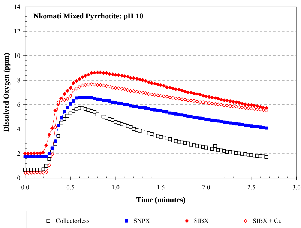
Figure 5.14: Change in dissolved oxygen with time for a slurry containing Nkomati MSB mixed pyrrhotite. Results are shown for the different reagent conditions at pH 10.
