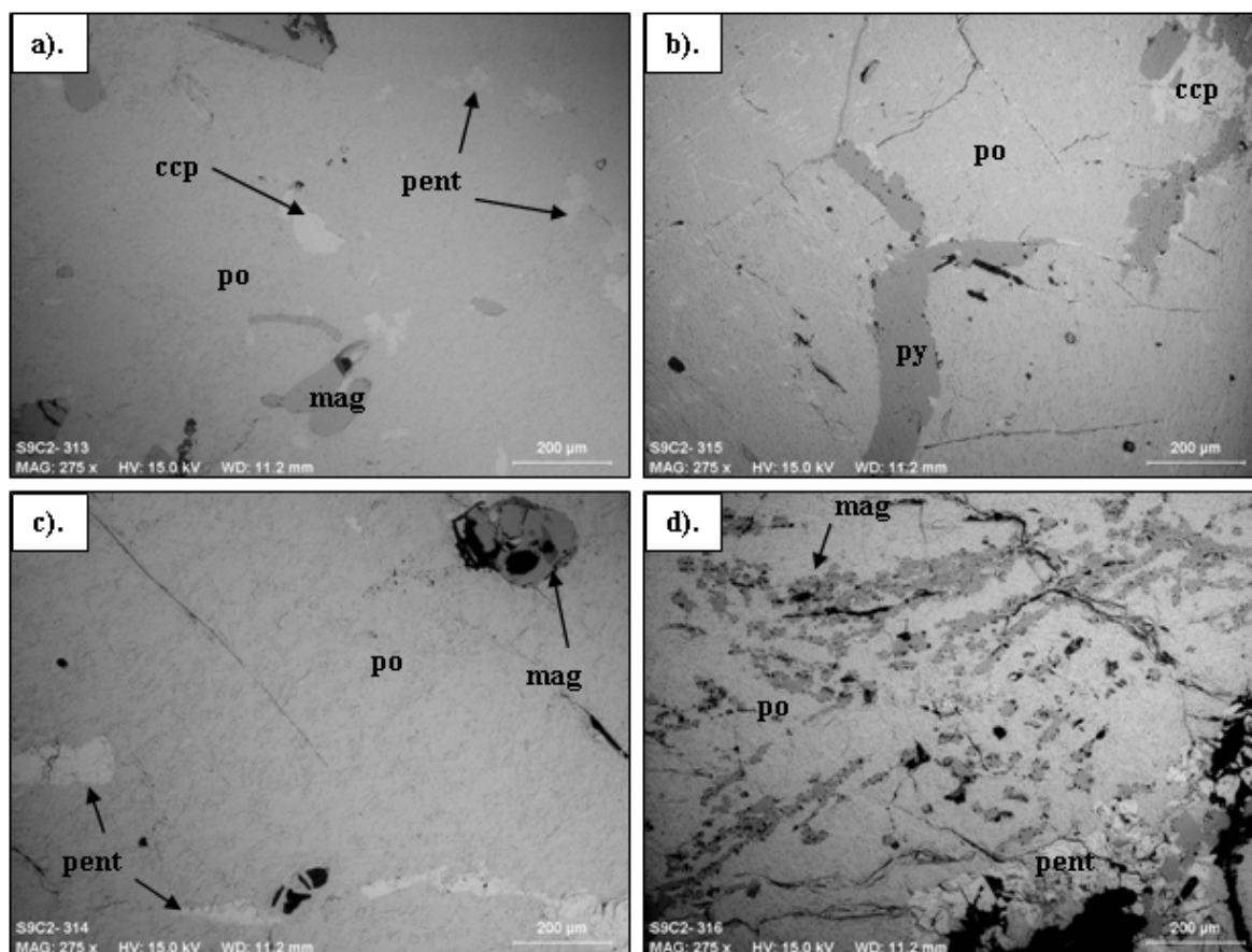
Figure 3.7: SEM BSE images of the pyrrhotite working electrodes used for electrochemical measurements. The contaminant minerals in the electrodes are shown. Images are shown for (a) Nkomati MSB mixed pyrrhotite (b) Phoenix magnetic pyrrhotite (c) Sudbury CCN non-magnetic pyrrhotite and (d) Sudbury Gertrude West magnetic pyrrhotite. Photograph courtesy of E. Bagci Tekes.
